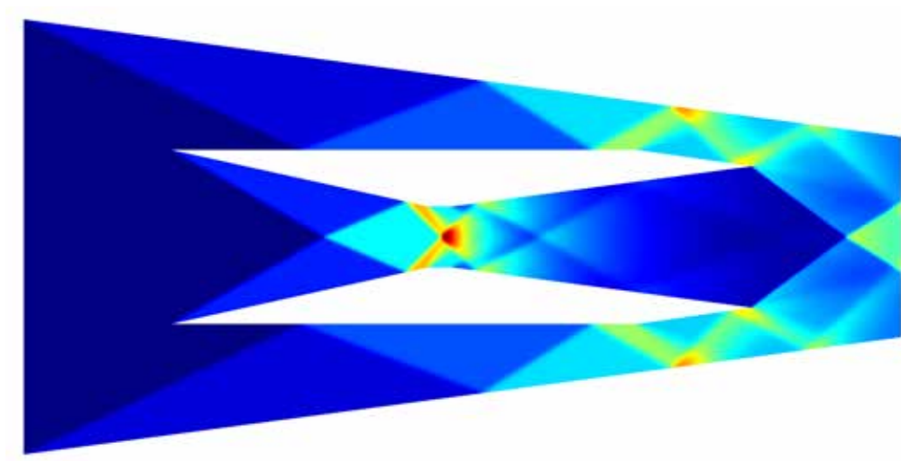
Accelerating Computational Fluid Dynamics (CFD) simulation on FPGA: shock waves in a 2D cross-section of a scramjet engine.
