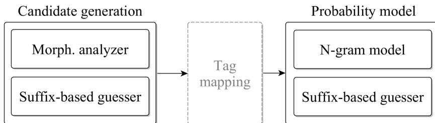
Figure 2.3 The data flow in the lemmatization component
