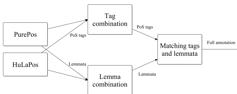
Figure 5.3 Combining the output of two PoS taggers and lemmatizers
