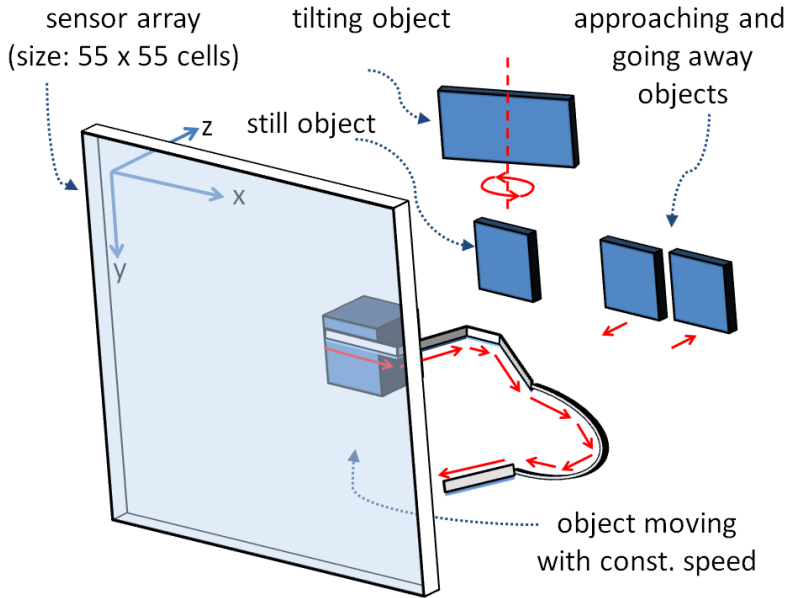
Figure 2: Simulation scene in connection with Thesis 2.2. In the scene we can see a standing object, a tilting object, a perpendicularly moving pair of objects (getting closer and going farther), and an object moving on a spatial trajectory at constant speed.
