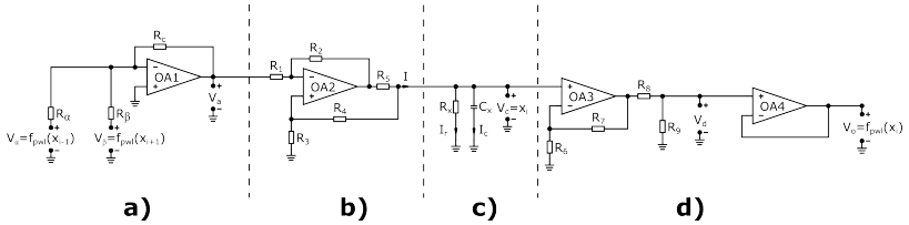
Figure 4: The schematic of a CNN cell built with the use of discrete components. The cell's functionality can be divided into four stages: summing amplifier (a), voltage controlled current source (b), inner state (c), and the realization of the piecewise linear output function (d) with a unity follower.
